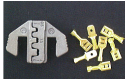
C DIE Open Barrel Terminal AWG 20-18/16-14/12-10 0.5-1.0/1.5-2.5/4.0-6.0 mm 2
