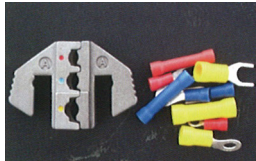
A DIE Insulated Terminal AWG 22-18/16-14/12-10 0.5-1.0/1.5-2.5/4.0-6.0 mm 2
