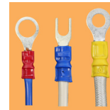
KC-8A4 For Insulated Terminal & Connector AWG 26-20/18-16/14/12-10 0.14-0.5/0.75-1.5/2.5/3.5-6 mm 2
