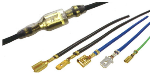
Open Barrel Connector (Non-Insulated Receptacle)
