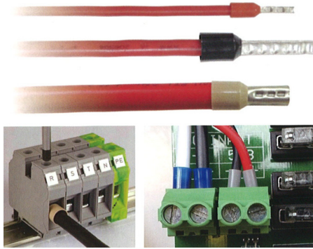
Cord End
