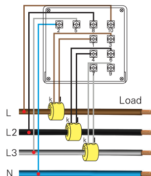
CONNECTION DIAGRAMS
