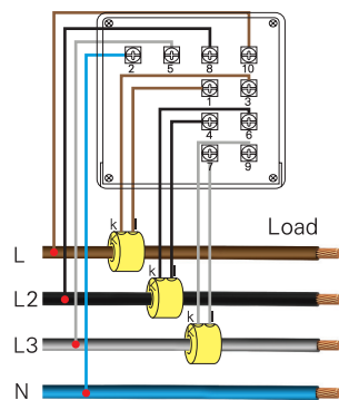
CONNECTION DIAGRAMS
